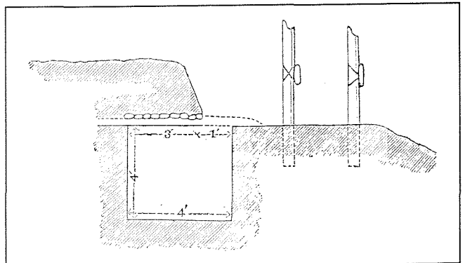
Fig. 12: Cross-section of a rifle pit. (Pasley 1863:587).
