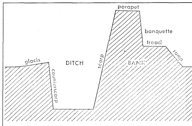
Fig. 14: Cross-section of redoubt defences.
